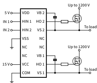
Typical connection
