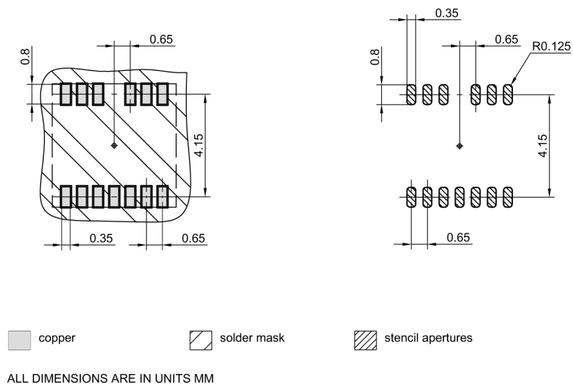
Figure 23 PG-TFLGA-13-1 footprint
