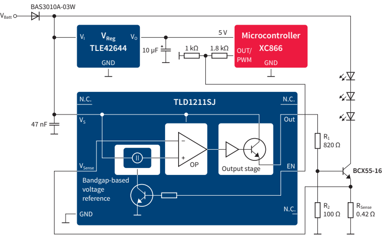
Application diagram TLD1211SJ
