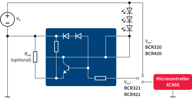
Block diagram BCR42x-U
